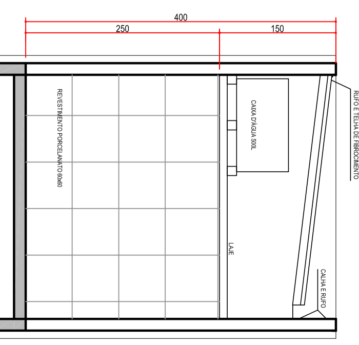
CORTE . IS ESC 1/50
